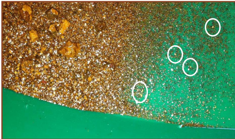
Figure 8. Crushed Iron pisolith sample containing gold grading up to 282 g/t in iron pisolites. (Source: TRP)
